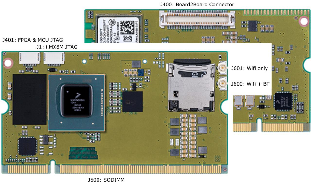
Figure 1-1: Connectors
