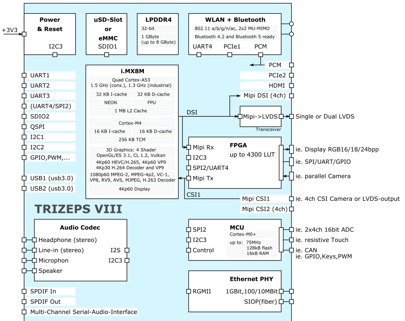
Figure 0-1: Simplified Block Diagram of Trizeps VIII
